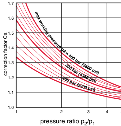
Correction factor C_a Adiabatic change of condition
