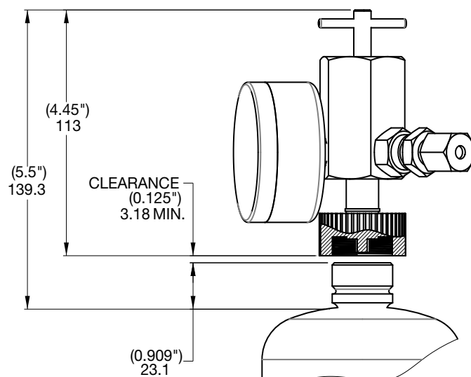
Diaphragm (SBO), Version 1 Gas Valve (M28 x 1.5) FPS Charging & Gauging Kit
