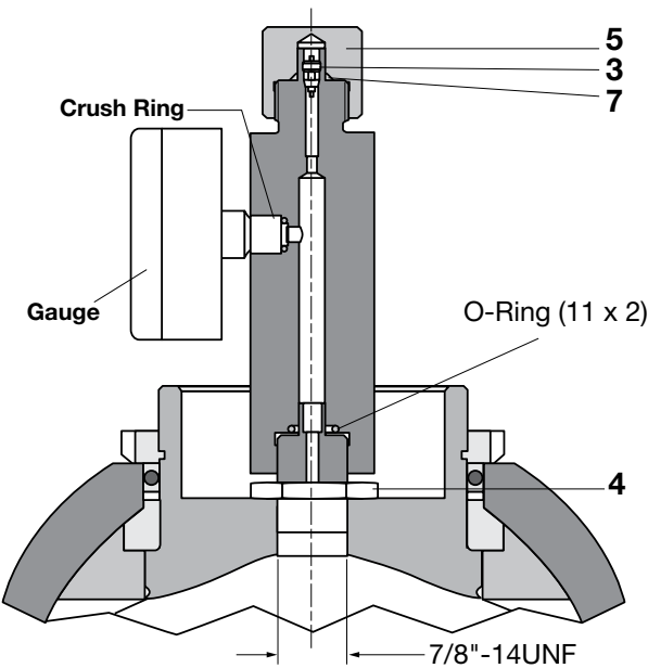
Top Repairable Bladder
