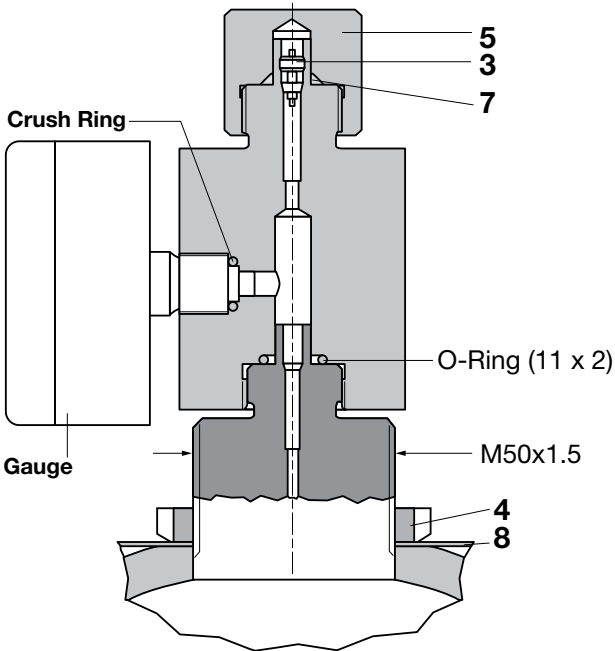
Bottom Repairable Bladder with M50 Gas Valve
